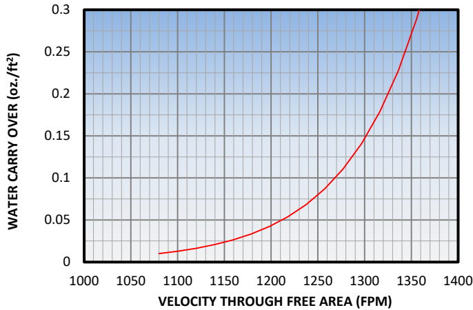
WATER PENETRATION - 2630 / 2635 15 MINUTE DURATION, TEST SIZE 48" x 48"
