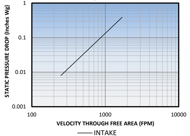
PRESSURE DROP - 2630 / 2635 FIGURE 5.5, TEST SIZE 48" x 48"
